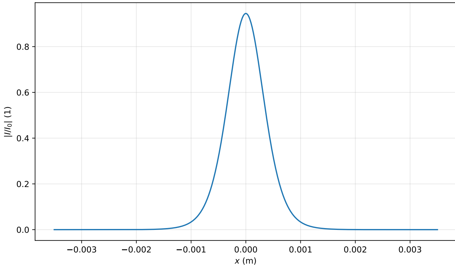
Intensity profile I(x, y = 0, z = 1.990m)/I_0 , P_{in}=0.6P_{cr} , artificial time
